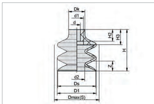
TGB-32至88
